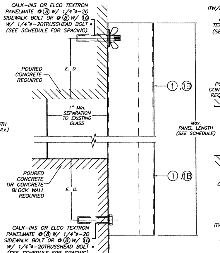
WALL MOUNTING INSTALLATION (D. M.) SECTION 2
