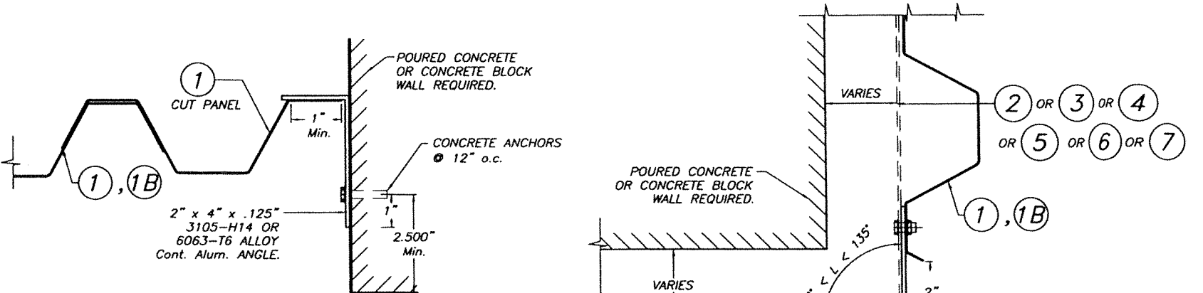
CASE A (Plan)
