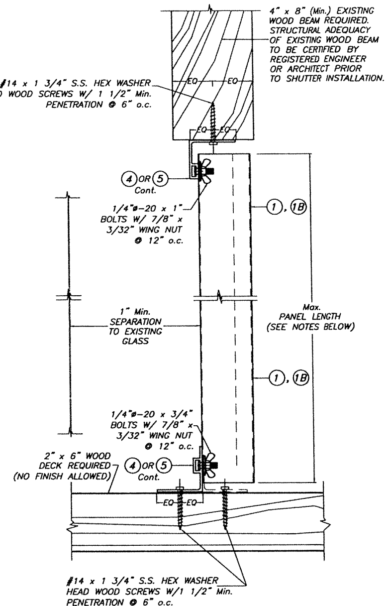
CEILING & FLOOR MOUNTING INSTALLATION ALTERNATIVE 6
