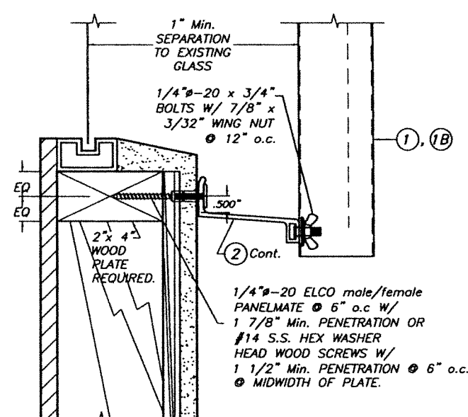
BUILD OUT INSTALLATION ALTERNATIVE 5
