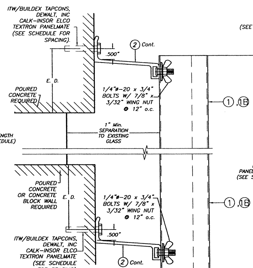
BUILD OUT INSTALLATION SECTION 3
