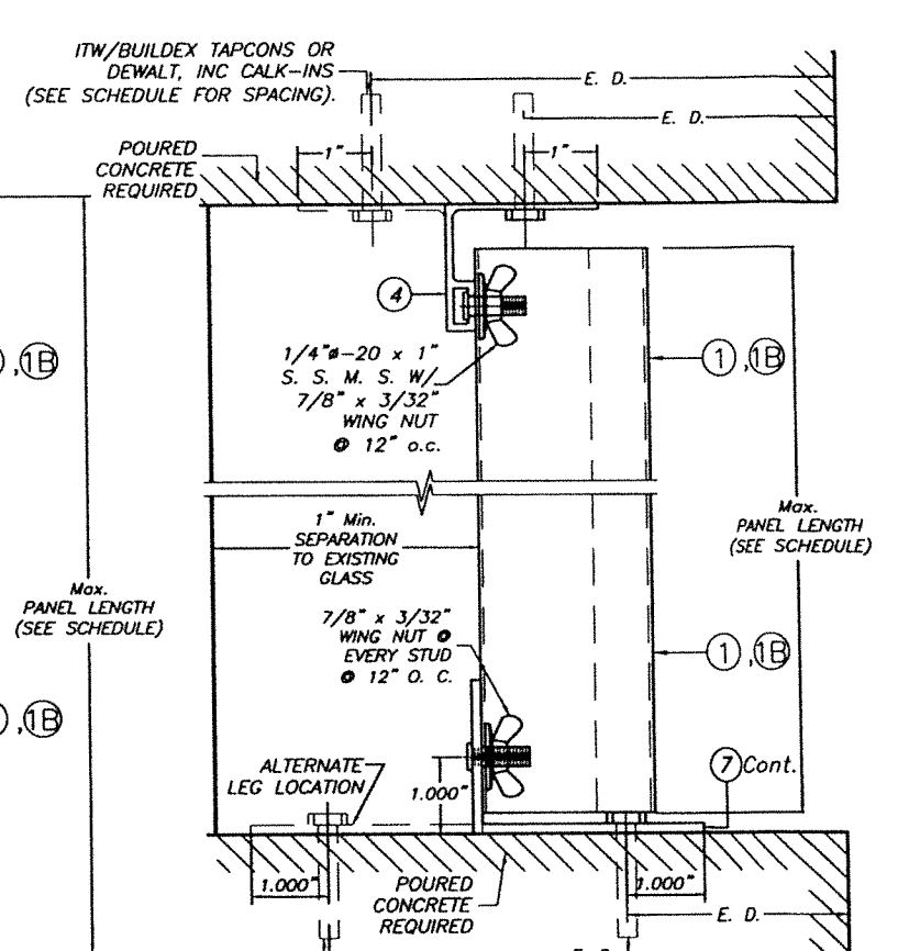
CEILING & FLOOR MOUNTING INSTALLATION SECTION 4
