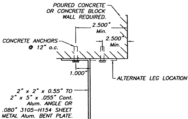
CASE A (Plan)
