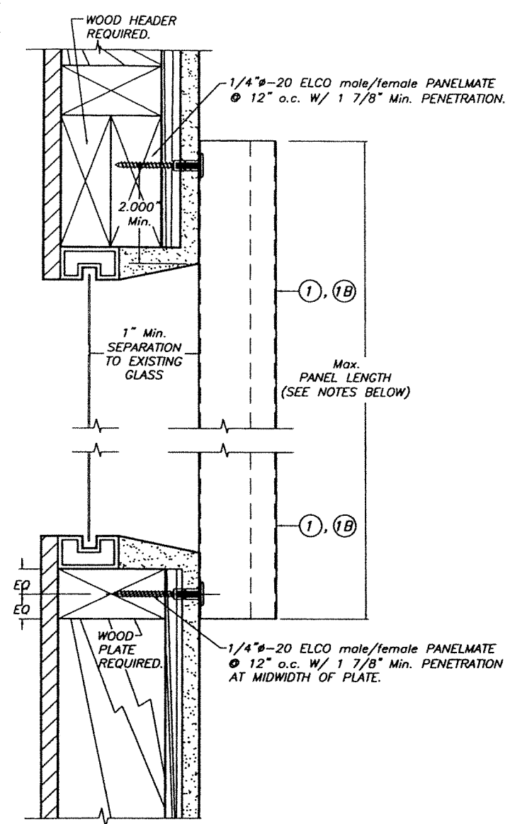
WALL MOUNTING (D. M.) ALTERNATIVE 1
