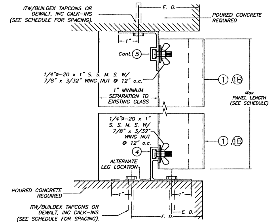
CEILING & FLOOR MOUNTING INSTALLATION SECTION 5
