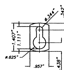
⑨ KEY HOLE WASHER 3105-H154 Alum. ALLOY
